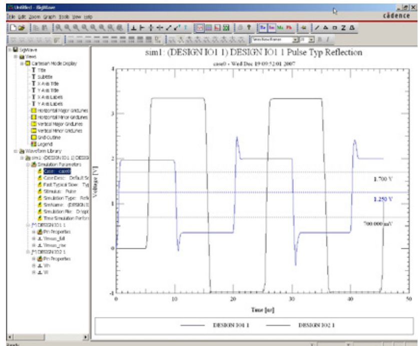
Figure 2: View and analyze simulation results in SigWave
