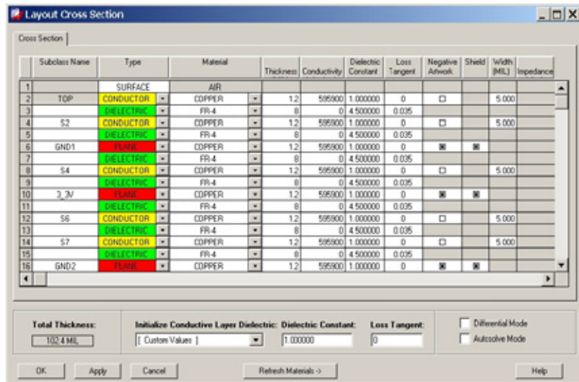
Figure 3: Change topologies or stack-up information to perform quick, iterative tradeoffs
