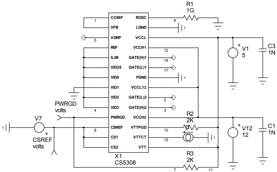
Figure 5.2.1 POWER GOOD SPICE Schematic
