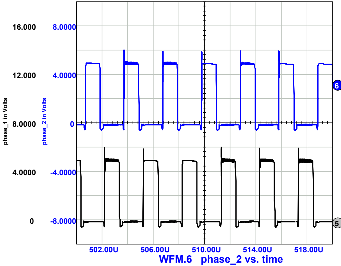
Figure 5.4.3 Spice Application Output Waveforms Top to bottom: PHASE2, PHASE1
