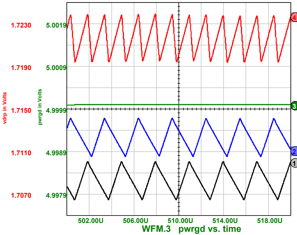
Figure 5.4.4 Spice Application Output Waveforms Top to bottom: VDRP, PWRGD, CS2-CSREF, CS1-CSREF
