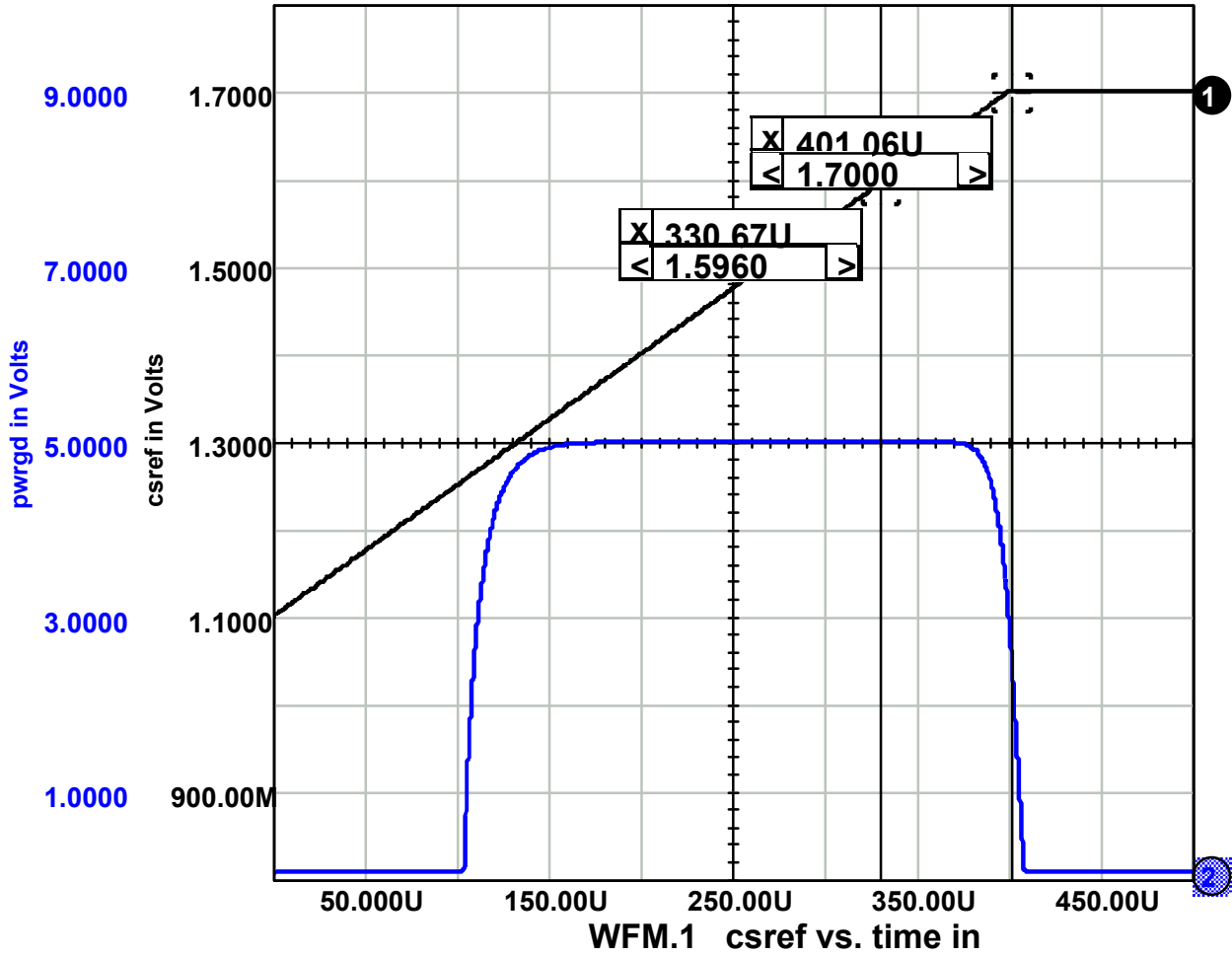
Figure 5.2.2: Power Good Spice waveforms
