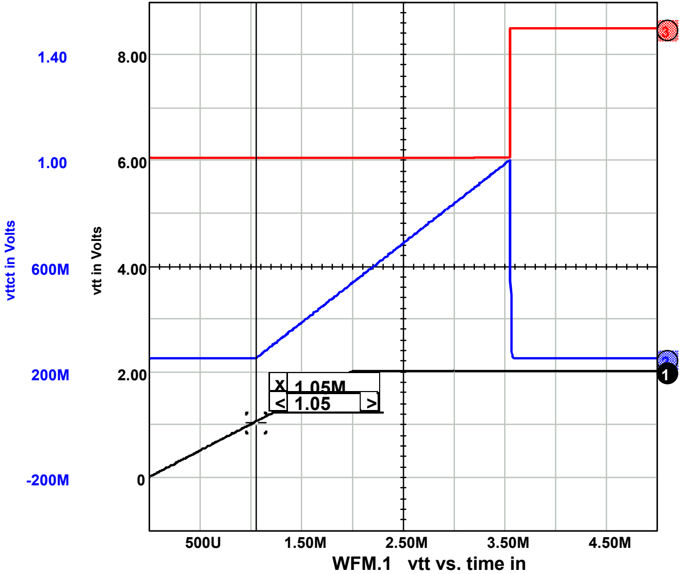
Figure 5.3.2 VTT GOOD SPICE Waveforms
