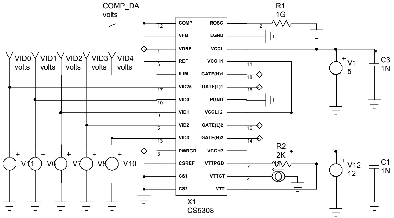
Figure 5.1.1 DAC Spice schematic
