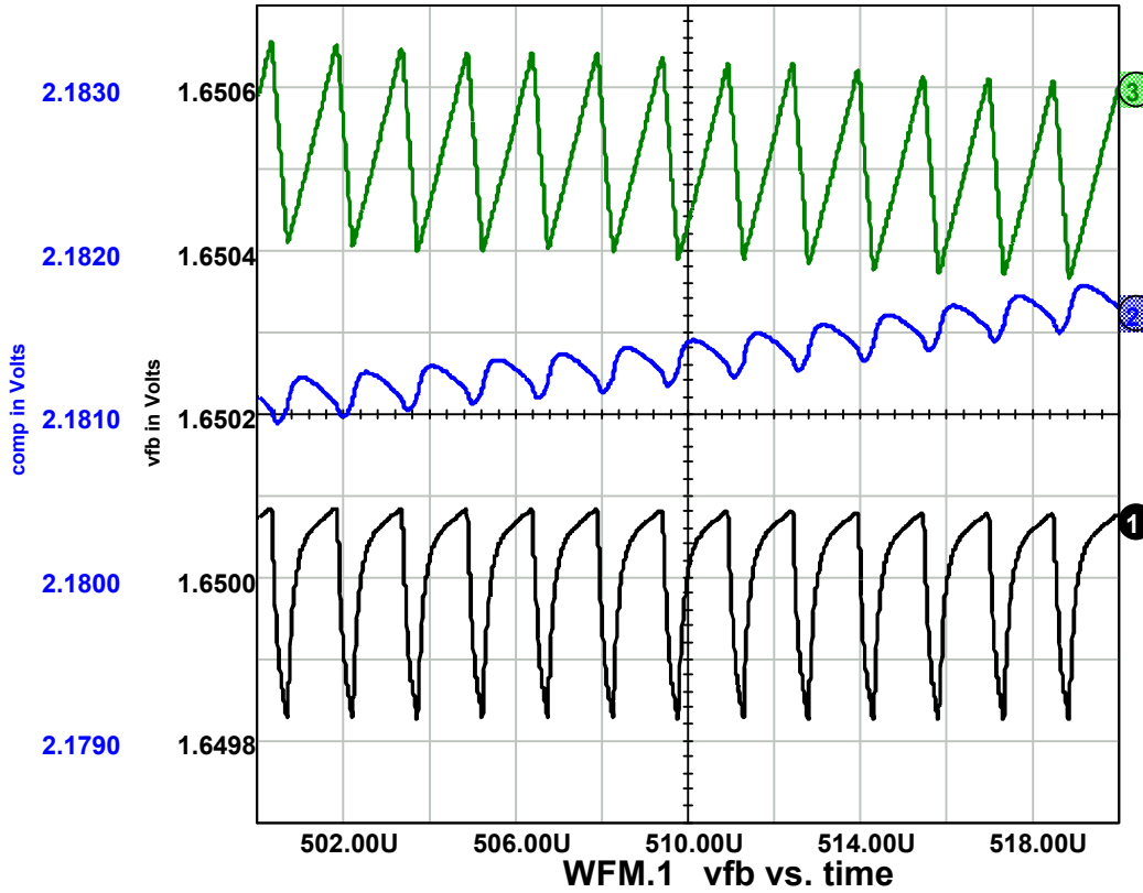
Figure 5.4.5 Spice Application Output Waveforms Top to bottom: VOUT, COMP, VFB
