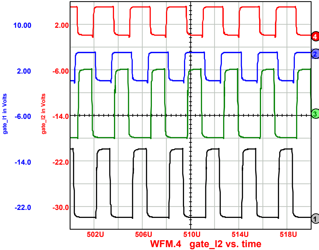
Figure 5.4.2 Spice Application Output Waveforms Top to bottom: GATE(L)2, GATE(L)1, GATE(H)2, GATE(H)1
