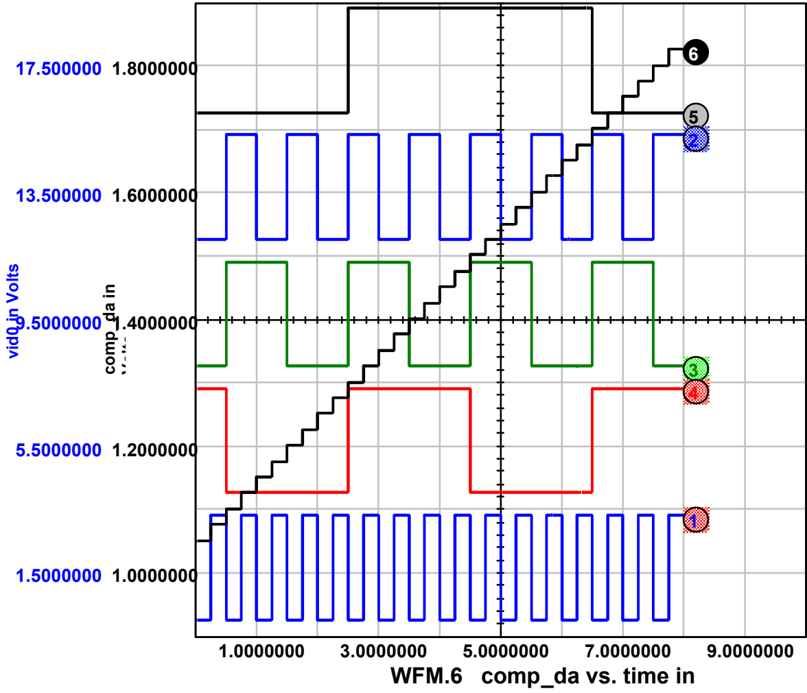
Figure 5.1.2 DAC Output SPICE Waveforms
