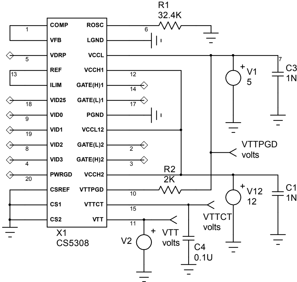
Figure 5.3.1 VTT GOOD SPICE Schematic
