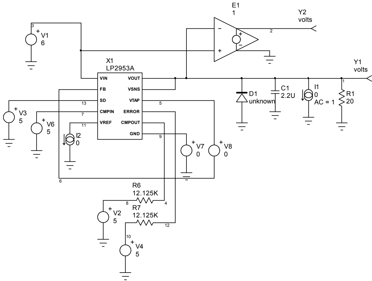
SPICE test circuit for manufacturer’s test conditions
