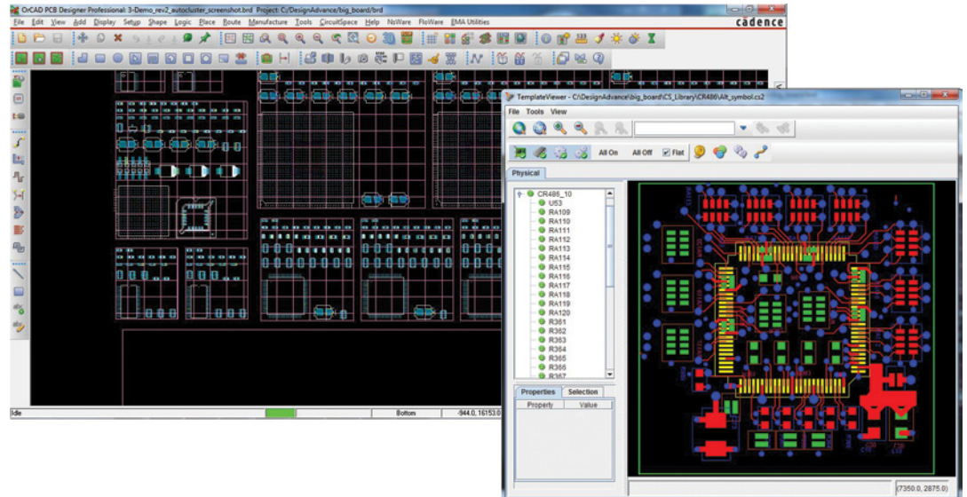
CircuitSpace allows for easy and flexible reuse of circuitry from design to design with layout templates. A viewer is included to preview available templates before applying them to the design.
