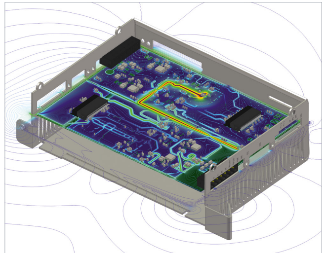
Radiated emissions: Fields from a PCB in an enclosure.
