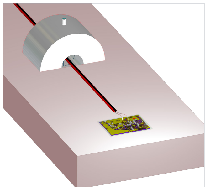
Bulk-current injection: Simulation of a BCI test of a PCB.
