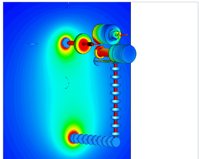
Electrostatic discharge: Surface current distribution of a highly-detailed model of an ESD generator.
