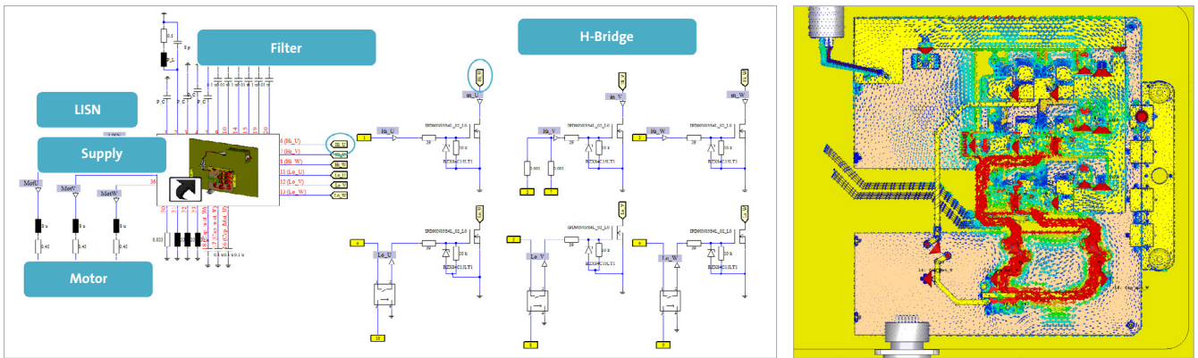
Conducted emissions: A variable frequency drive (VFD) motor control, showing the circuit level representation (left) and 3D surface currents (right).
